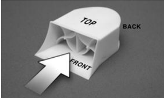
84 VorBlade™ vortex generators (several extra generators may be included)
