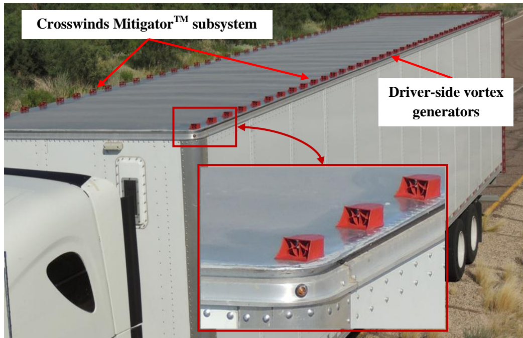
Crosswinds Mitigator™ subsystem on a typical 53' trailer
